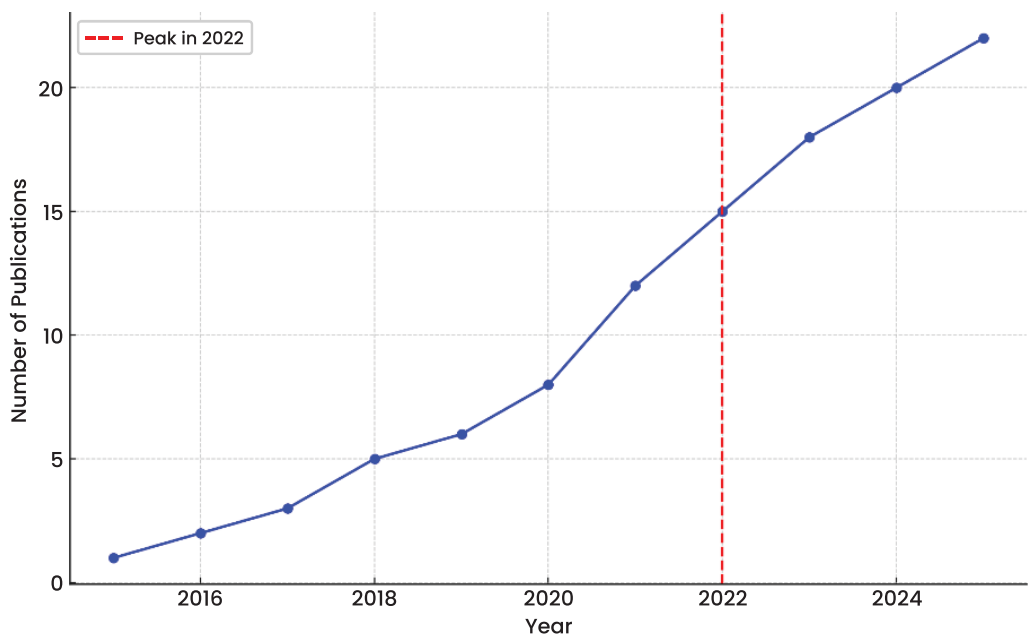
Fig. (3). Timeline of publications on tunable topological edge states (2015-2025).
