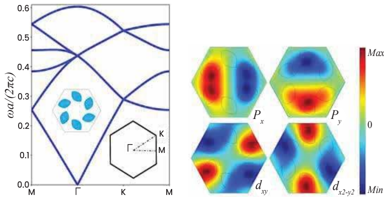
Fig. (2). Band structure for the TM modes (Source: [29]).
