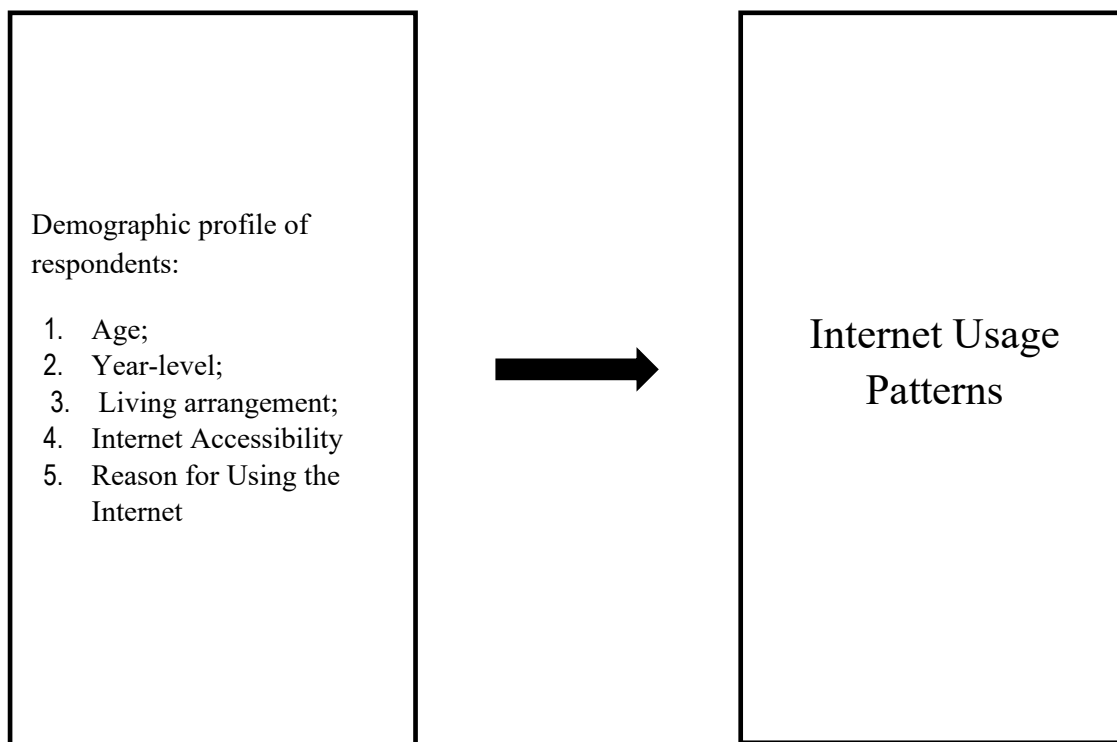
Fig. (1). Paradigm showing the independent variables and dependent variables.
